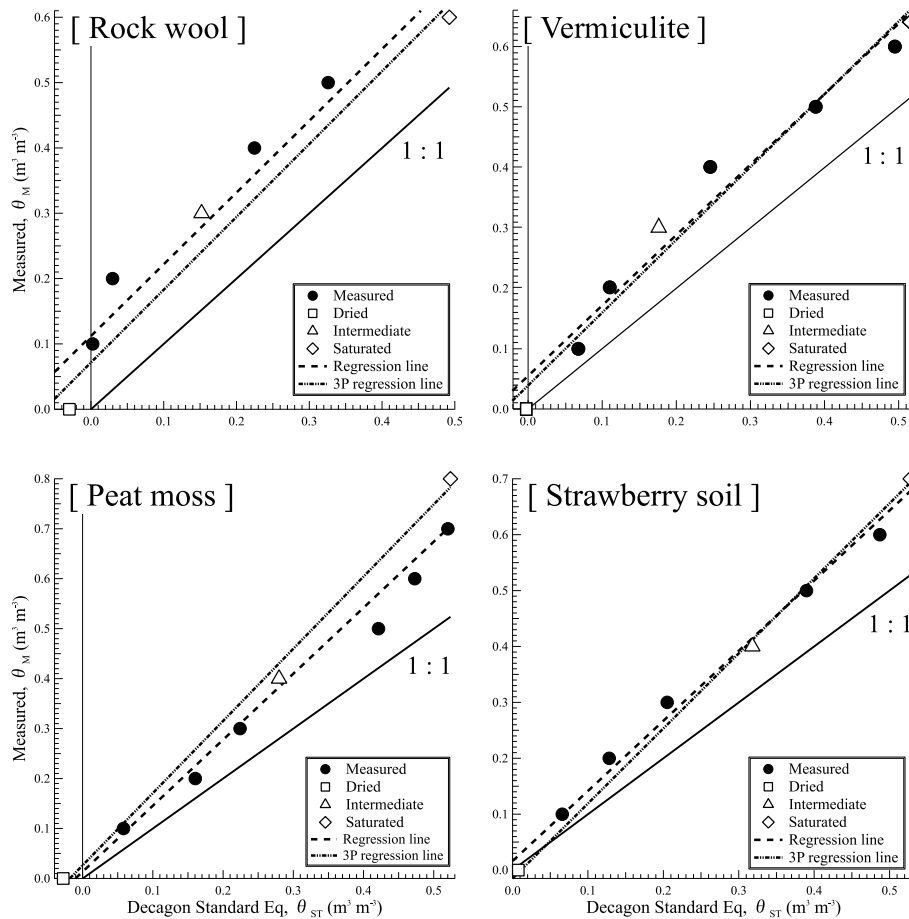
Fig. 2 4 種類の農業用培地の GS3 の標準式で求めた \theta_{ST} と重量測定に基づく \theta_M の関係 (●). 実線は \theta_{ST} の 1 : 1 直線. 破線は \theta_{ST} と \theta_M の一回帰直線. 二点鎖線は 3 点 (乾燥 : □, 中間 : △, 飽和 : ◇) の \theta_{ST} と \theta_M から求めた一回帰直線. The relationship between volumetric water content \theta_{ST} based on the standard equation and gravimetrically measured \theta_M for four type of agricultural materials. The solid line shows 1:1 relationship and the broken line is a regression line between \theta_{ST} and \theta_M . The two-dot chain line is a regression line for three water content samples (dried, intermediate, and saturated).
